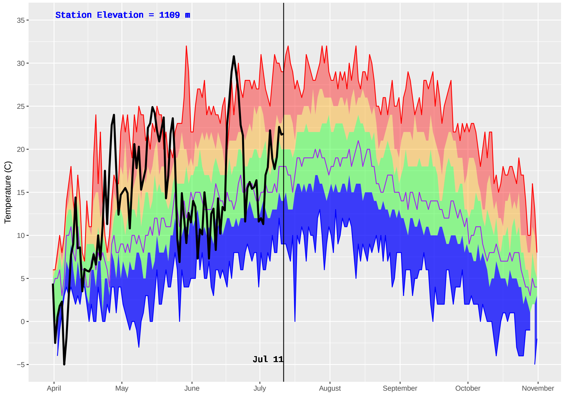
MOOSE LAKE (165) : Historical (1980–2016) and Current (2018) Noon Temperature
