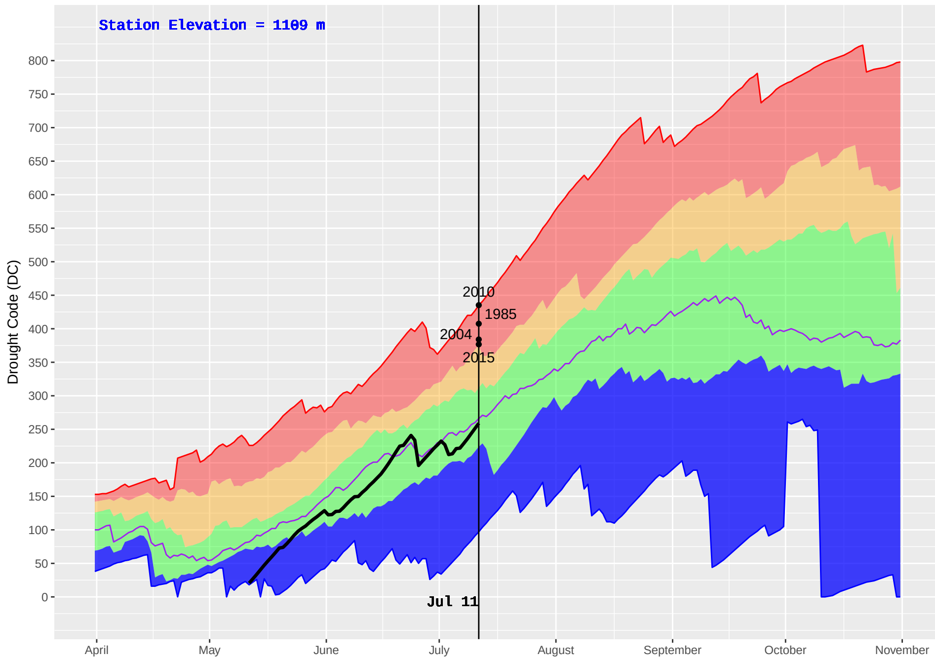
MOOSE LAKE (165) : Historical (1980–2016) and Current (2018) Noon Drought Code (DC)
