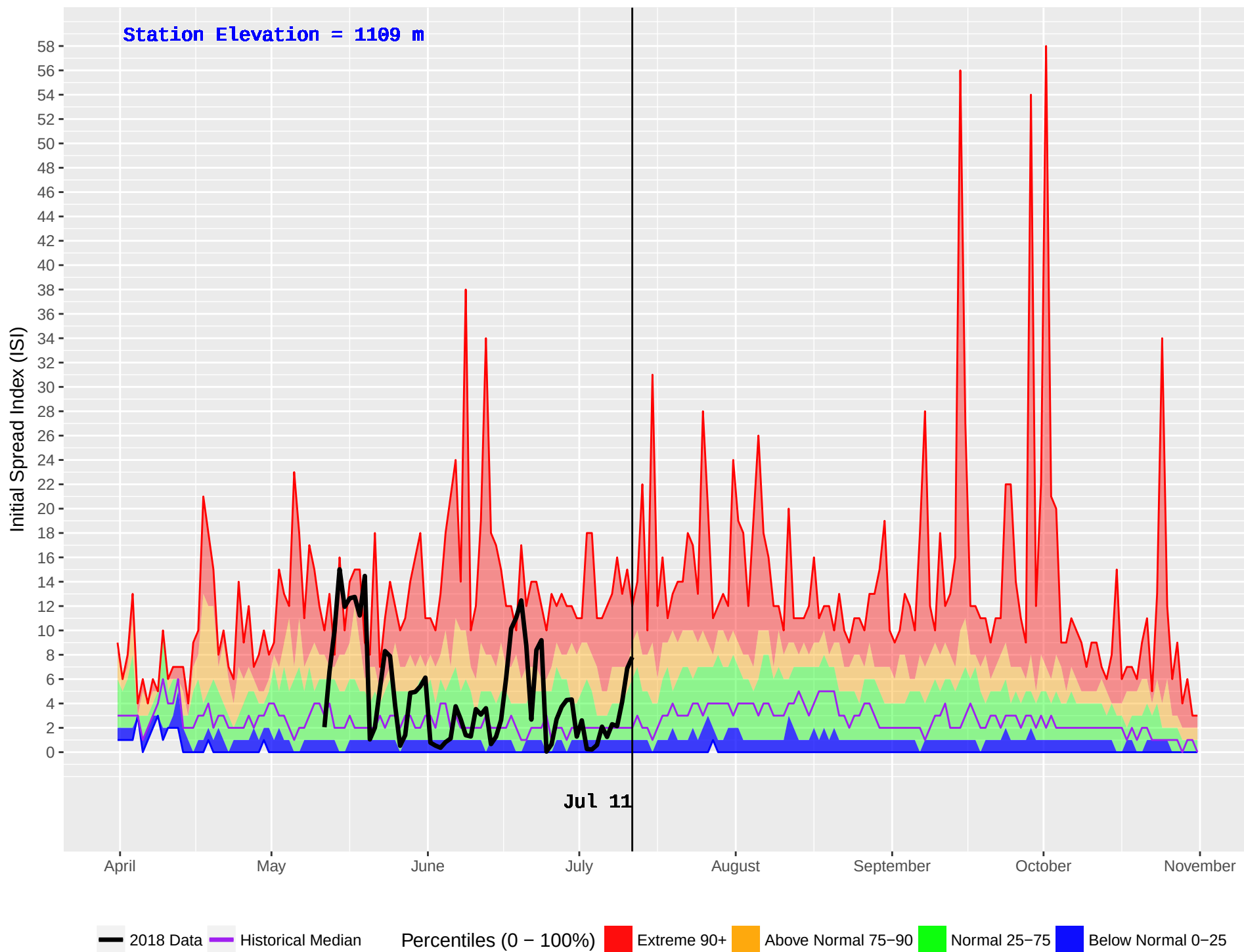
MOOSE LAKE (165) : Historical (1980–2016) and Current (2018) Noon Initial Spread Index (ISI)
