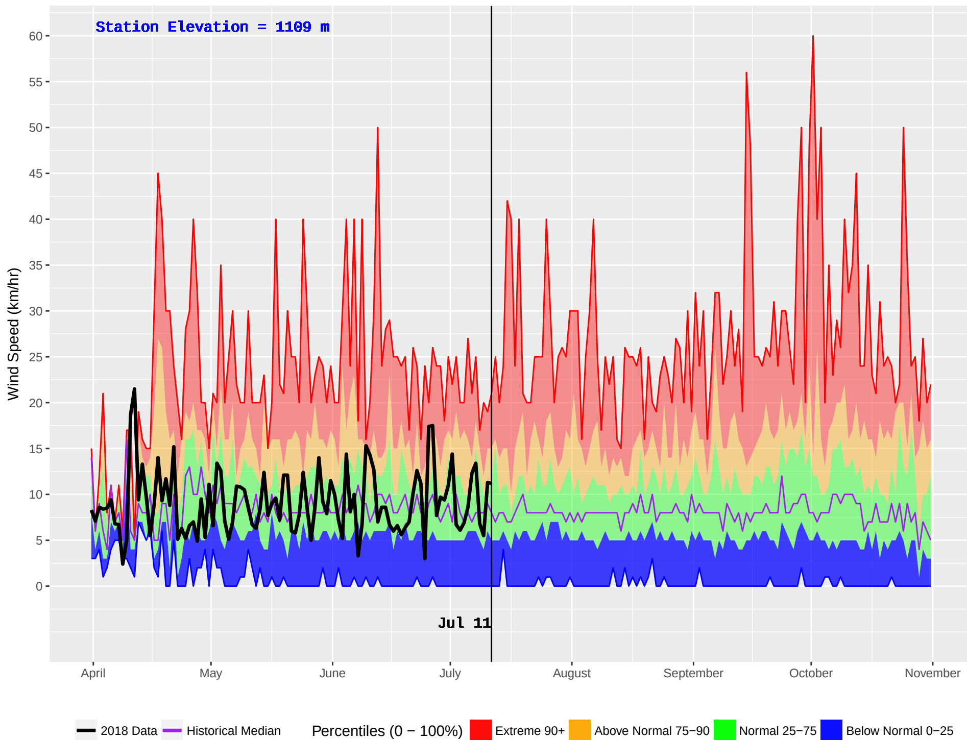
MOOSE LAKE (165) : Historical (1980–2016) and Current (2018) Noon Wind Speed
