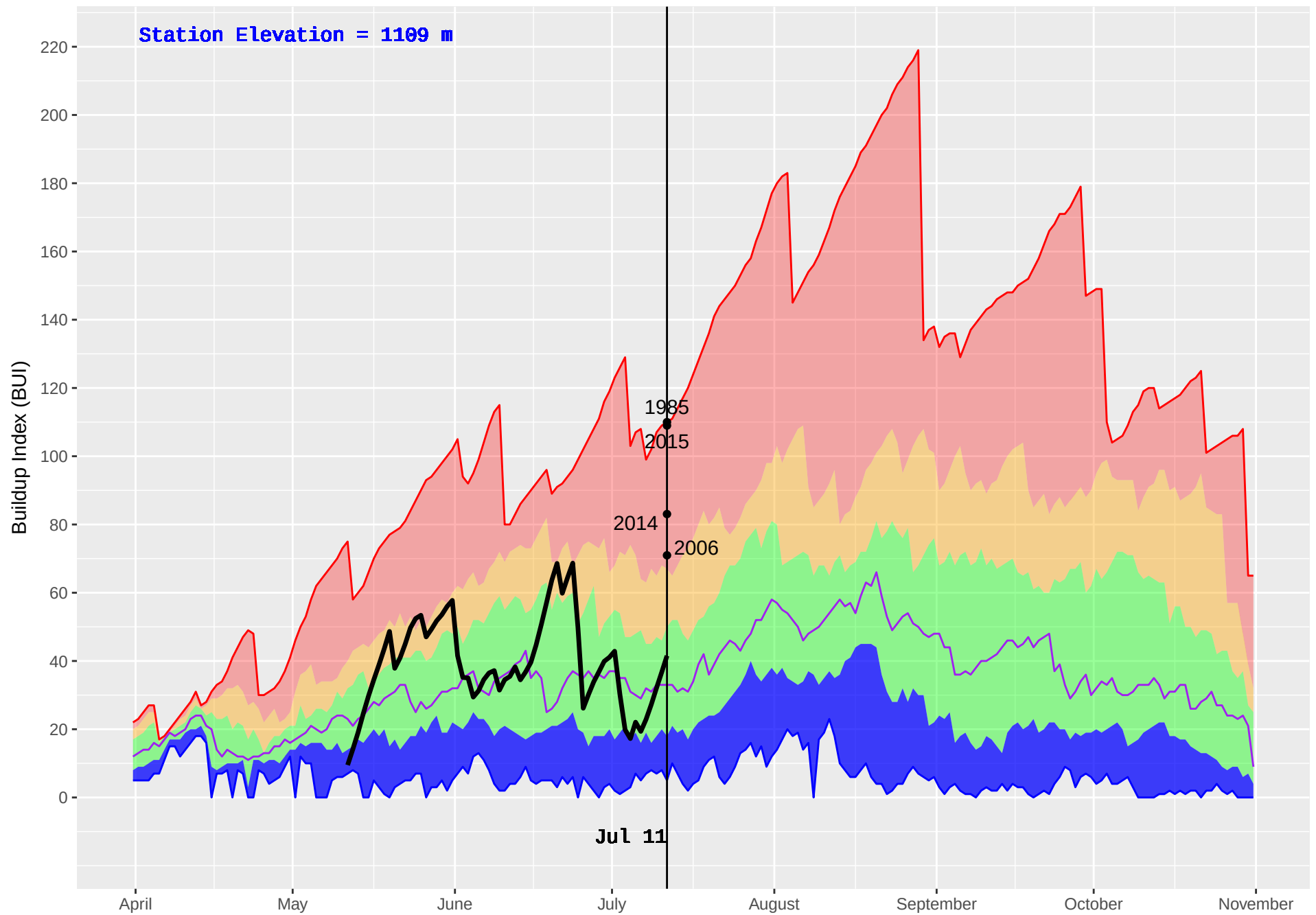
MOOSE LAKE (165) : Historical (1980–2016) and Current (2018) Noon Buildup Index (BUI)
